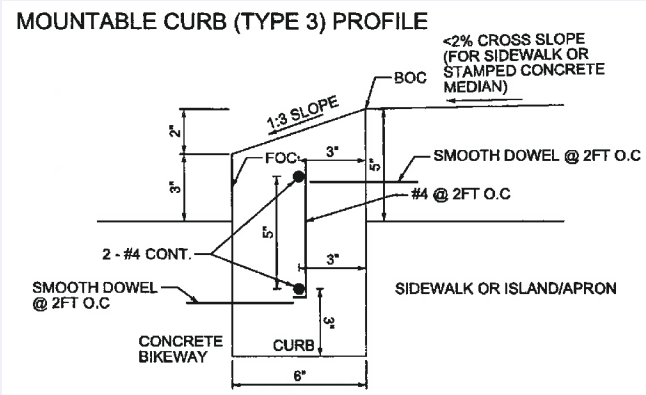
The mountable curb features a 3 inch (75 mm) vertical rise followed by a further 2 inch (50 mm) over 6 inch (150 mm) run for a 1:3 slope. Image: City of Austin.
