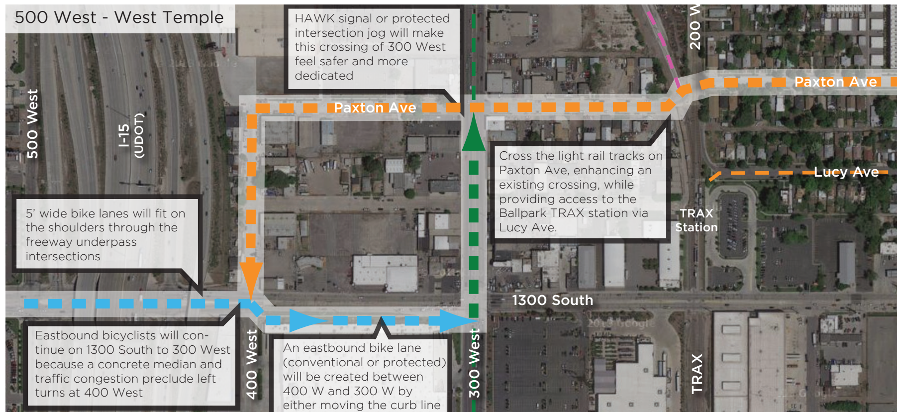
Figure 6-10 1300 South Interim Bypass Route
