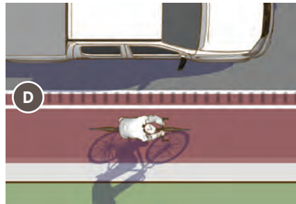
Figure 3-3. Longitudinal markings along shoulders should be selected in response to shoulder width, and the desire to discourage encroachment by motor vehicles.
