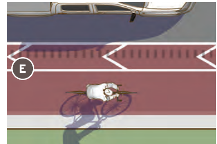
Figure 3-3. Longitudinal markings along shoulders should be selected in response to shoulder width, and the desire to discourage encroachment by motor vehicles.
