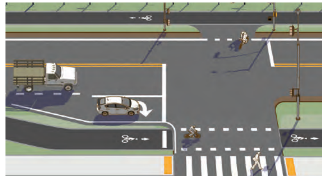
Figure 4-22. A variety of design treatments exist depending on the roadway configuration, available curb-to-curb width, traffic volumes and desire to provide a dedicated turn lane. All designs should strive to reduce speeds of turning vehicles, remind users of bicycle priority, and clarify user positioning up to and through the intersection.
