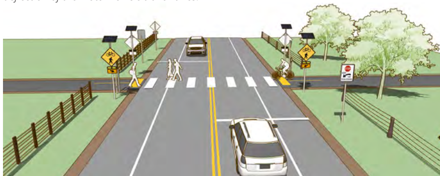
Figure 4-6. Where yield compliance is low, rectangular rapid flash beacons can be used to draw attention to crossing path users and signal their intent to cross.
