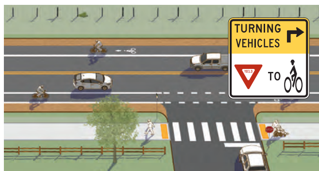
Figure 3-10. A variety of design treatments exist depending on the roadway configuration, available curb-to-curb width, traffic volumes and desire to provide a dedicated turn lane. All designs should strive to reduce speeds of turning vehicles, remind users of bicycle priority, and clarify user positioning approaching and through the intersection. Common signs at intersections include R4-4 Begin Right Turn Lane Yield to Bikes and a modified R10-15 Turning Vehicles Yield to Bikes sign. (1)
