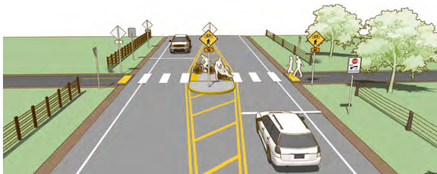
Figure 4-5. A median safety island should allow path users to cross one lane of traffic at a time. The bicycle waiting area should be at least 8 ft deep to allow for a variety of bicycle types. To promote yielding to bicyclists the median safety island should be designed to require horizontal deflection of the motor vehicle travel lanes.
